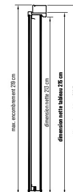
SECTION VERTICALE
